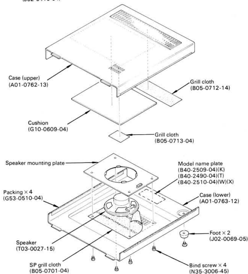
Fig. 12 Case disassembly
